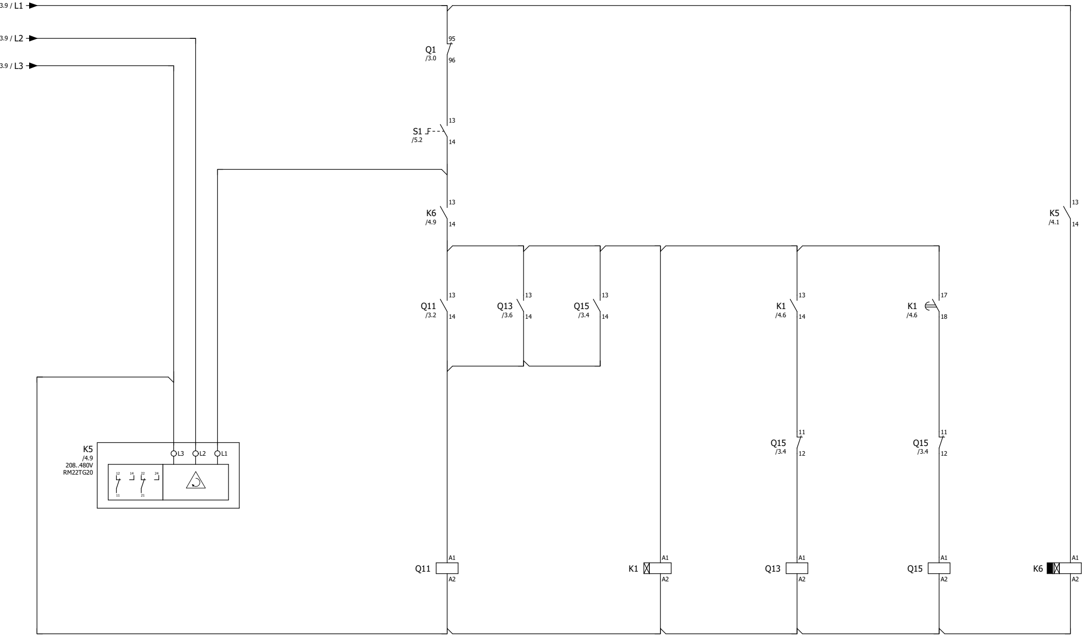
MAIN RELAY
