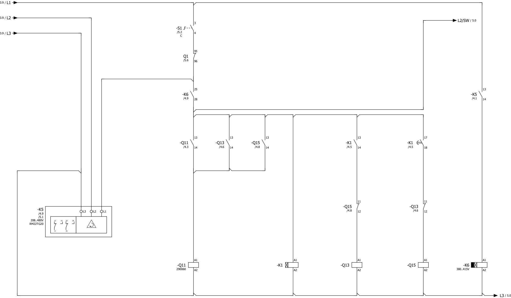
MAIN RELAY
